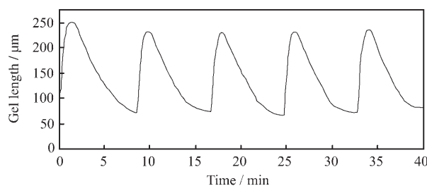
Figure 1. Oscillation profiles of cubic poly(NIPAAm-co-[Ru]-co-AMPS) gel. The cubic gel (length of each side ca. 0.5 mm) was immersed in a solution (1 mL) of the BZ substrates (malonic acid (62.5 mM), sodium bromate (84 mM), and nitric acid (0.894 M) at 18 °C).
